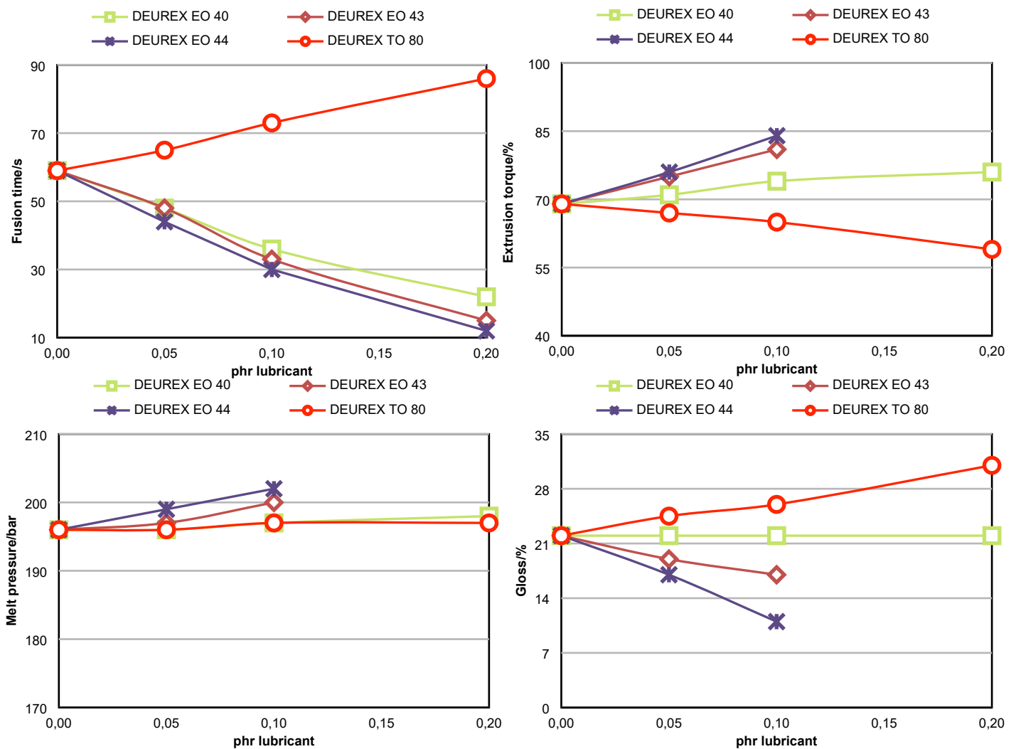
Fig. 1 to Fig. 4 Influence of the dosage of DEUREX® EO 43 in comparison to EO 40, EO 44 and TO 80 on fusion time (Fig. 1), extrusion torque (Fig. 2), melt pressure (Fig. 3) and gloss (Fig. 4)
